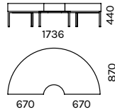
ZK-PK180-MJ
