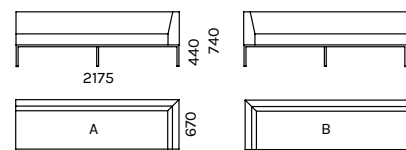
ZK-D3A-MJ, ZK-D3B-MJ
