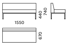
ZK-D2-MJ
