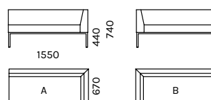
ZK-D2A-MJ, ZK-D2B-MJ
