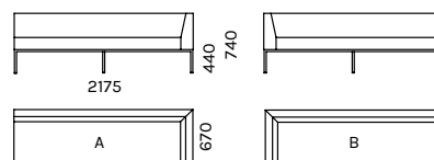
ZK-D3A-MJ, ZK-D3B-MJ
