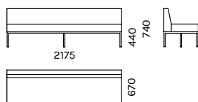
ZK-D3-MJ
