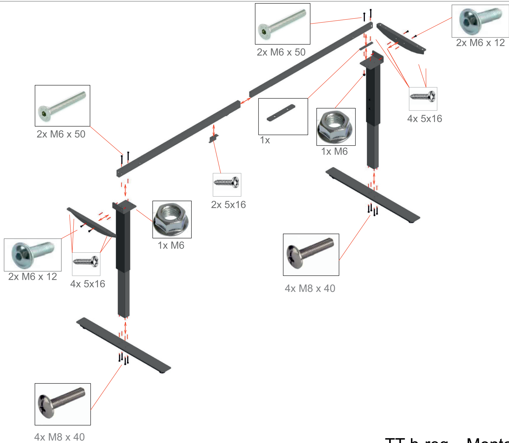
TT h-reg Montage drawing
