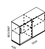
STORAGE CABINET SE4241
