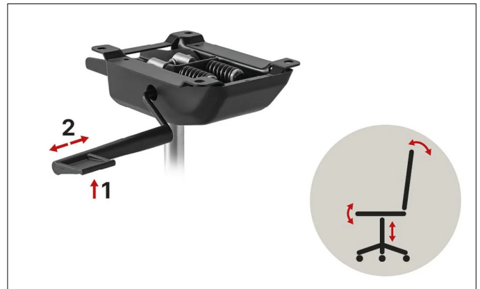
Self-weighting synchron (P) Seat and backrest tilt synchron mechanism with automatic tension adjustment and seat height adjustment
