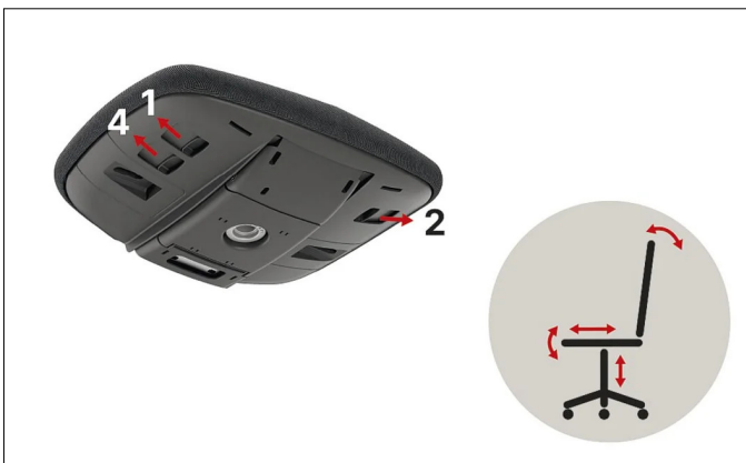
Synchron self-weighting slide system (F) For Advanced version. Seat and backrest synchron tilt mechanism integrated into the seat, with self-weighting tension adjustment, with seat height and seat depth adjustment
